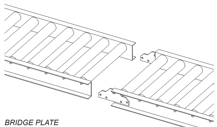
END COUPLER
